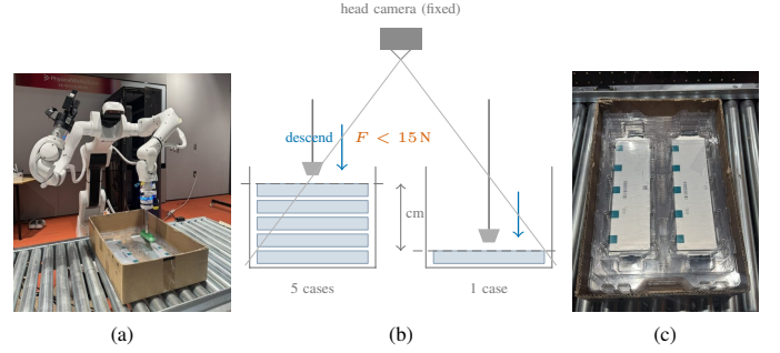
Fig. 1. Setting. (a) The dual-arm mobile manipulator picking a battery-cell case from a tray with a suction cup. (b) The stack height varies across episodes, so the contact plane moves by centimeters, while the head camera keeps the same pose; a few millimeters of over-travel take contact force past the 15 N limit. (c) The head-camera view of a tray: from this range the remaining stack height is visually near-indistinguishable across layers, so the stop-on-contact transition must be carried by force, not vision.
