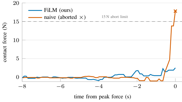
Fig. 4. Contact force on the robot: one representative trial per policy, aligned at peak force ( t=0 ), over the interaction window (before lift, where carrying the case would re-enter payload weight into the measured force). The naive attempt rises through the demonstrated range and is terminated by the external 15 N abort ( \times ; all three naive attempts end this way, at 15.4–18.7 N), while the FiLM-policy pick presses to 2.5 N—the median of its nine picks across three stack heights, one of them absent from the demonstrations—and stops on its own.
