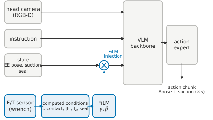
Fig. 2. The FiLM policy. The raw wrench does not enter the policy state; force reaches the action only as the computed condition vector \hat{c} , injected through FiLM modulation of the state token entering the VLM backbone. Because this pathway is explicit and unique, forcing \hat{c} at inference measures the causal authority of the condition.
