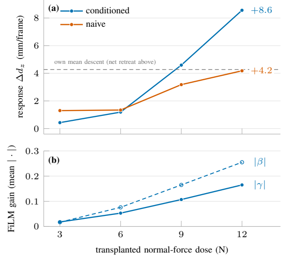
Fig. 4. On-robot counterfactuals (P5): identical frozen observations, wrench transplanted to a fixed normal-force dose. (a) The response ordering reverses between 6 and 9 N—the offline crossover on the physical system. (b) FiLM modulation magnitude rises monotonically with dose.
