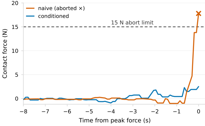
Fig. 3. Contact force on the robot: one representative trial per policy, aligned at peak force ( t=0 ), over the interaction window (before lift, where carrying the case would re-enter payload weight into the measured force). The naive attempt rises through the demonstrated range and is terminated by the external 15 N abort ( \times ; all three naive attempts end this way, at 15.4–18.7 N), while the conditioned pick presses to 2.5 N—the median of its nine picks across three stack heights, one of them absent from the demonstrations—and stops on its own.
