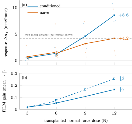
Fig. 4. On-robot counterfactuals (P5): identical frozen observations, wrench transplanted to a fixed normal-force dose (circles: ten-pose session; squares: three-pose session; faint dots: individual poses). (a) The response ordering reverses between 6 and 9 N—the offline crossover on the physical system. (b) FiLM modulation magnitude rises monotonically with dose.
