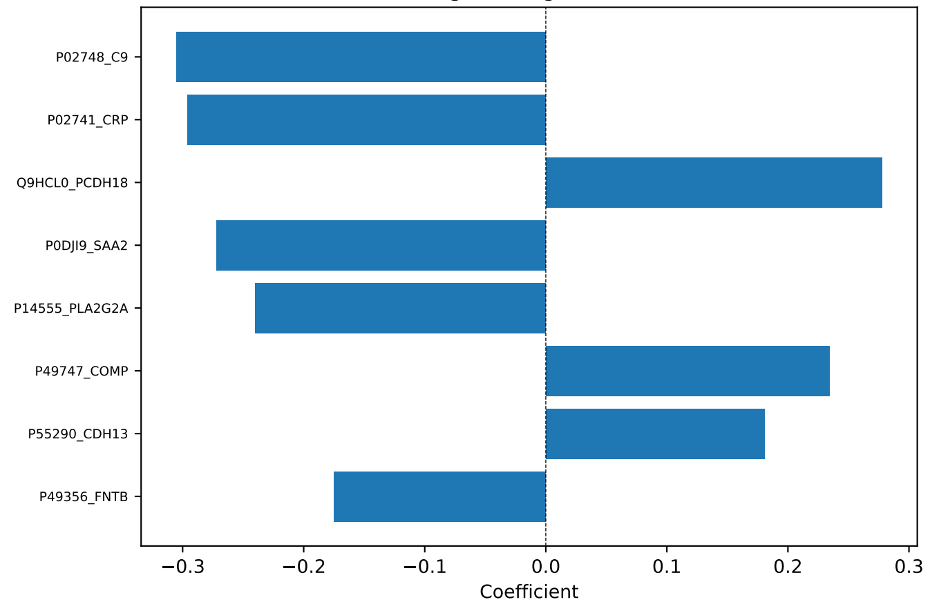
Logistic Regression
