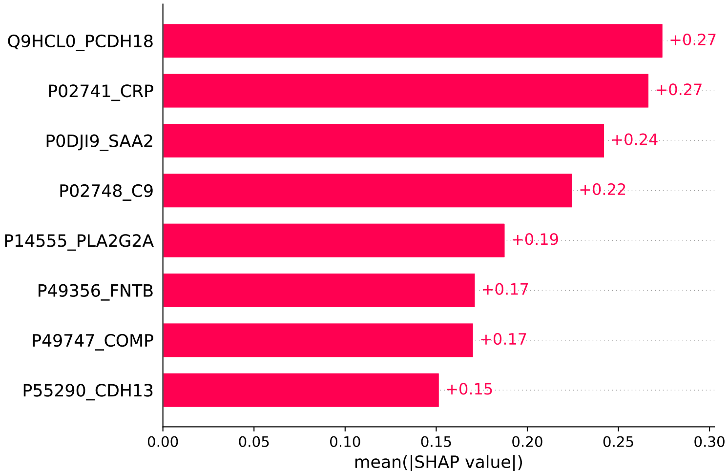
SHAP Feature Importance (Test, n=40)
