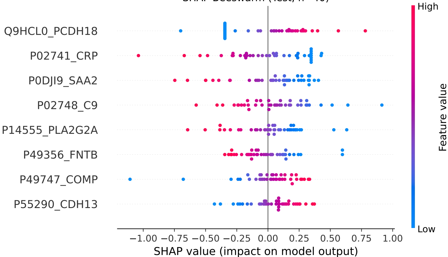
SHAP Beeswarm (Test, n=40)
