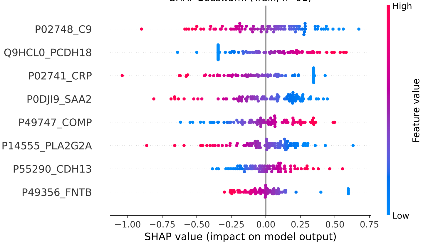
SHAP Beeswarm (Train, n=91)
