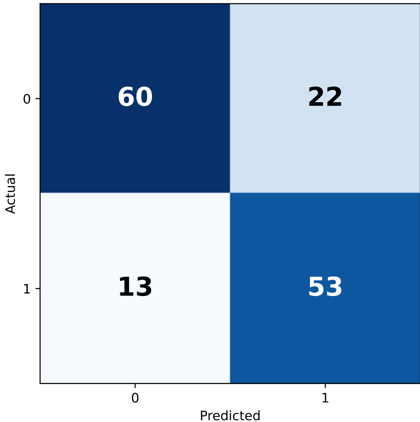
LR Validation Confusion Matrix
