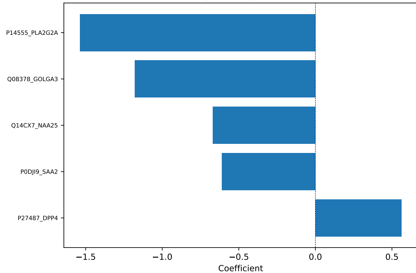
Logistic Regression
