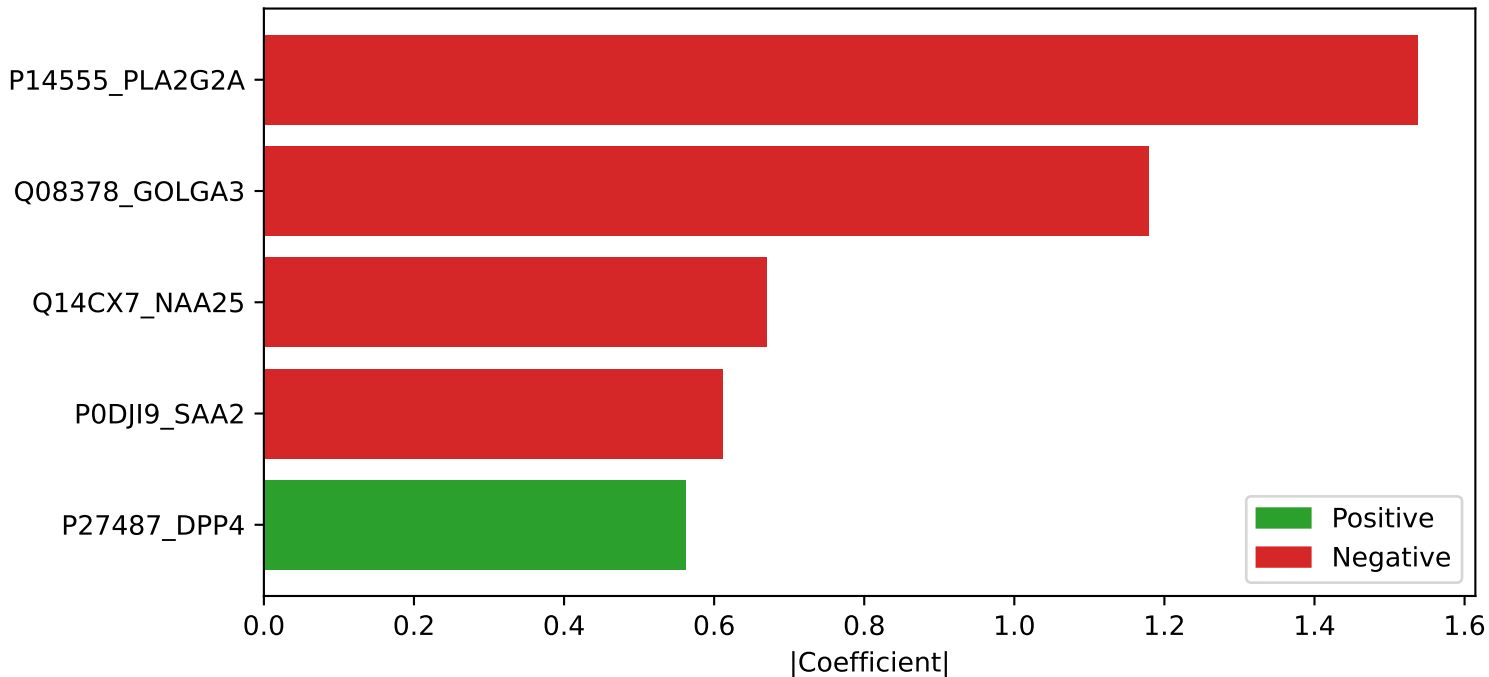
Logistic Regression Feature Importance (5 features)
