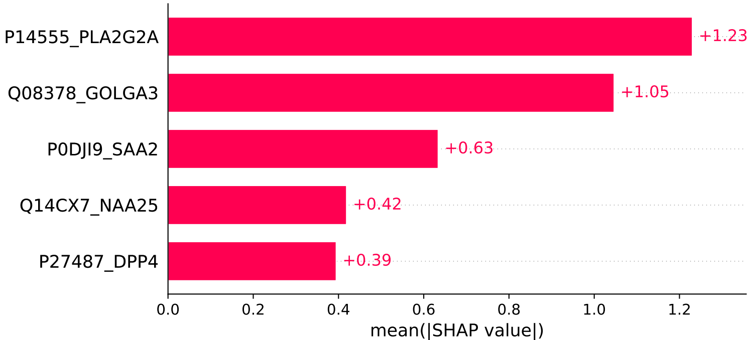
SHAP Feature Importance (Test, n=16)
