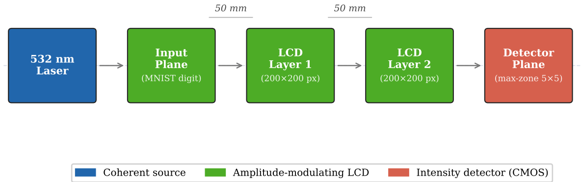
Fig. 1. System architecture of the two-layer LCD-based ONN.
