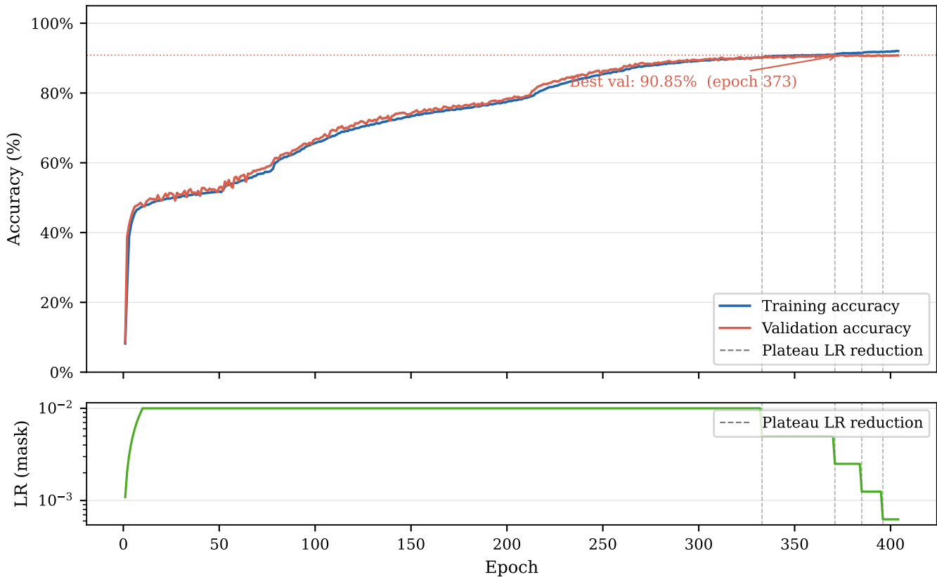
Fig. 3. Training and validation accuracy curves for the max-zone 5 \times 5 model over 403 epochs, with the learning rate schedule shown in the lower panel.
