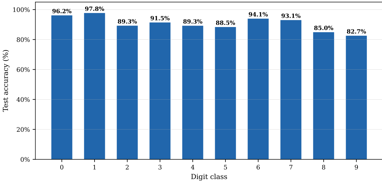
Fig. 4. Per-class test accuracy of the max-zone 5 \times 5 model on the 10,000-image MNIST test set.
