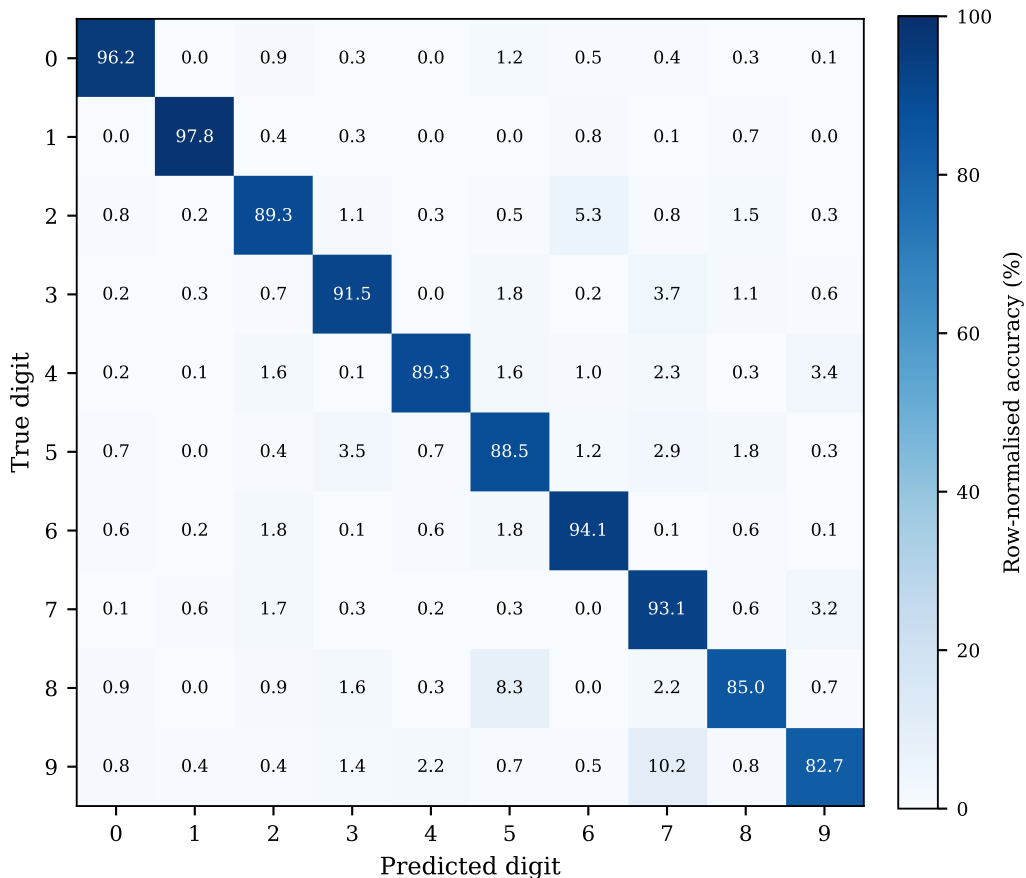
Fig. 5. Row-normalised confusion matrix for the max-zone 5 \times 5 model on the 10,000-image MNIST test set.
