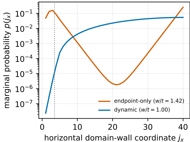
(b) Ground state at \delta E_m , L = 40
