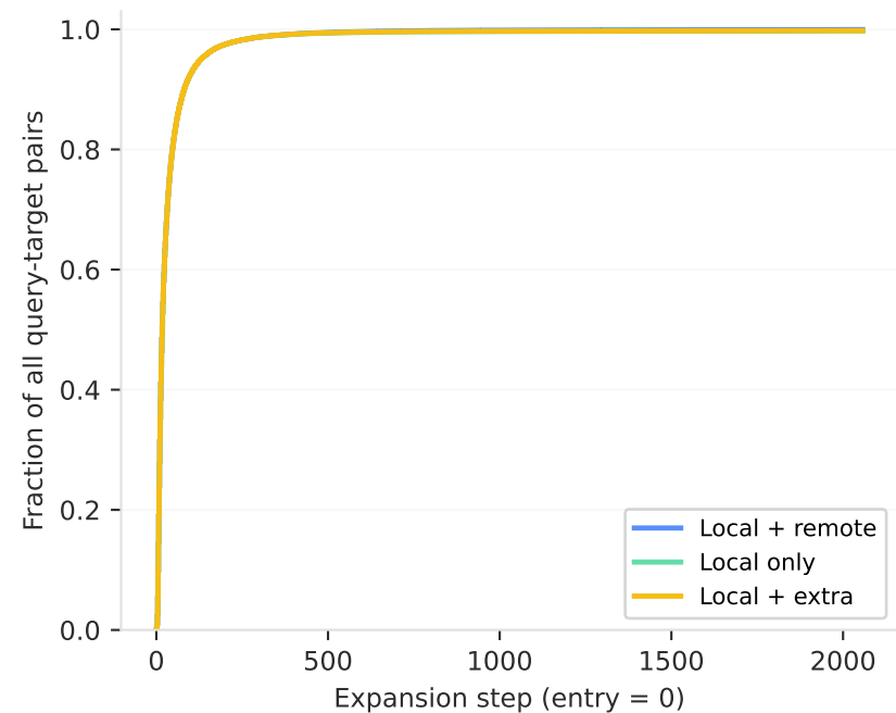
Discovery of ground-truth top-100
