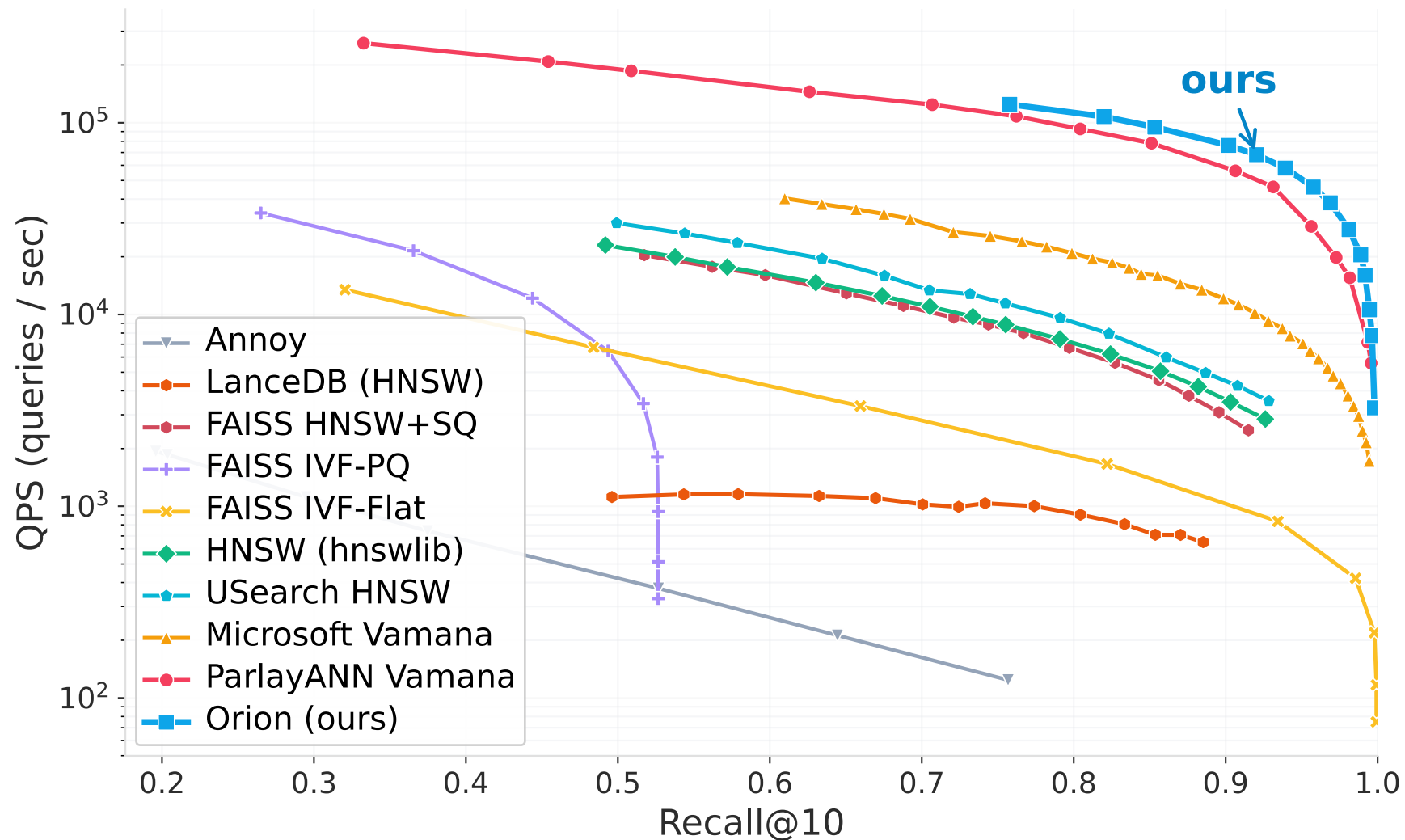
GIST 1M — QPS vs Recall@10 (8 threads, k=10)
