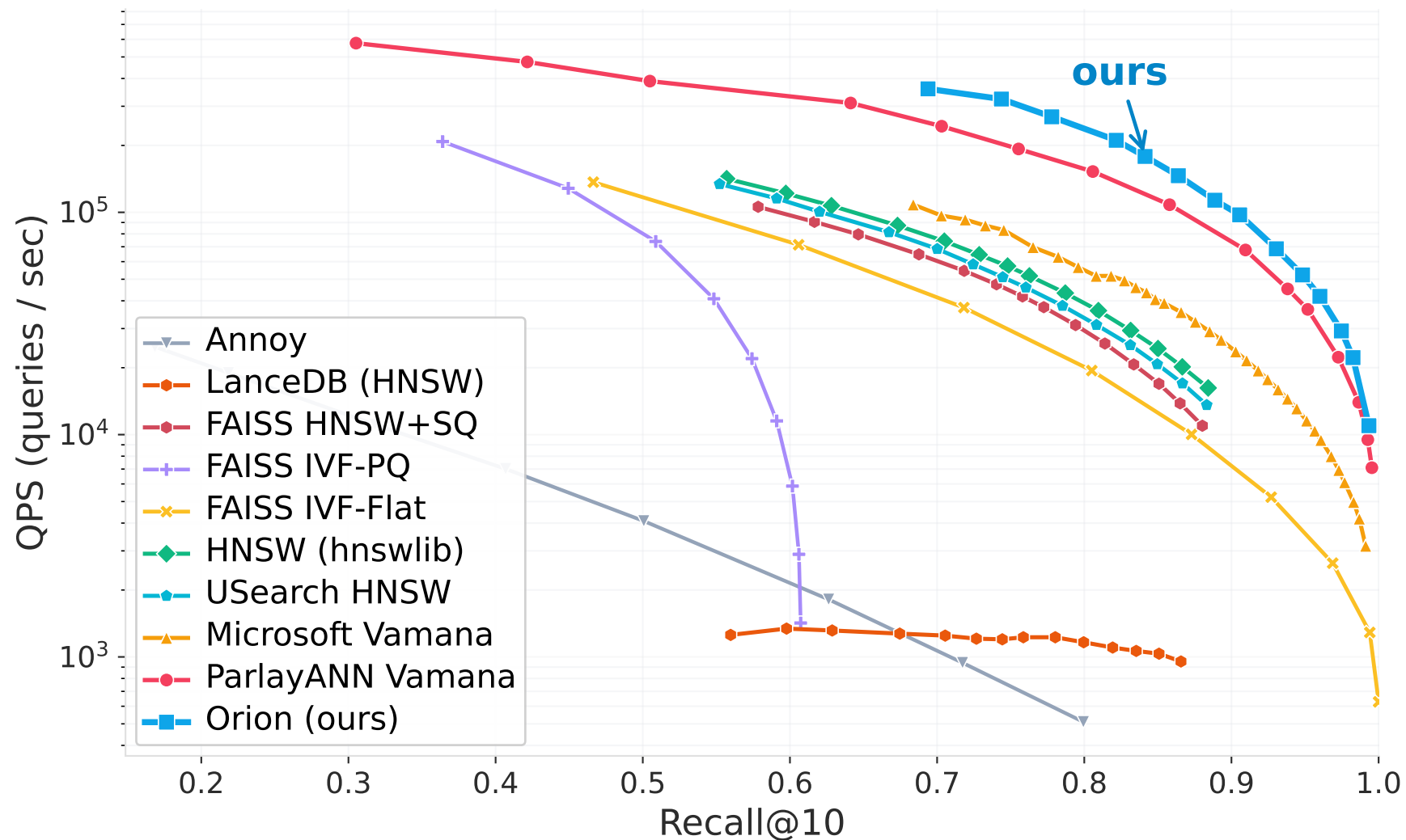
GloVe-100 (cosine) — QPS vs Recall@10 (8 threads, k=10)
