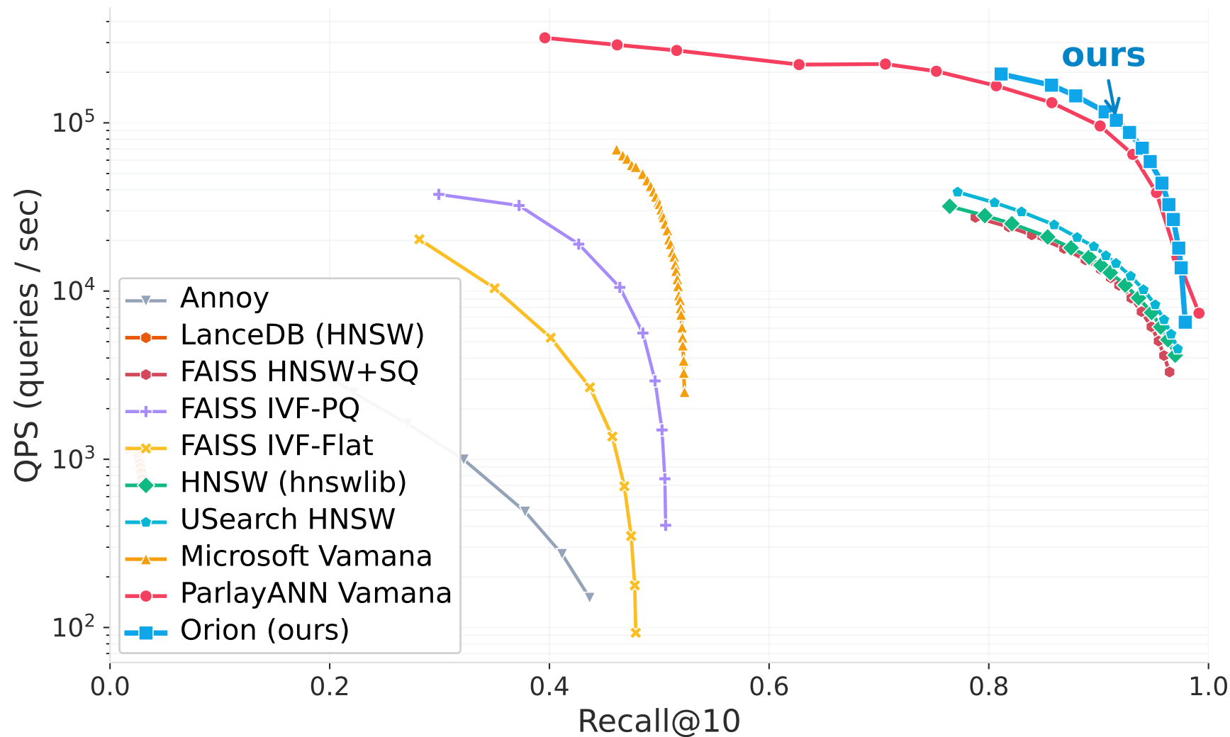
MS-MARCO BERT 1M (raw IP) — QPS vs Recall@10 (8 threads, k=10)
