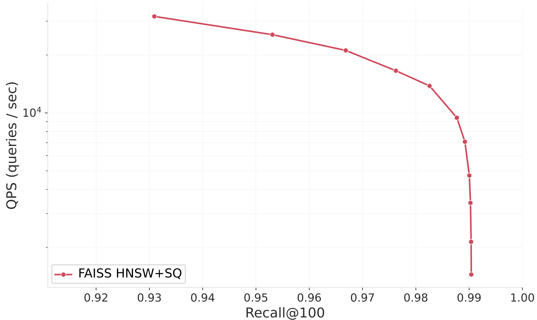
SIFT 1M — QPS vs Recall@100 (8 threads, k=100)
