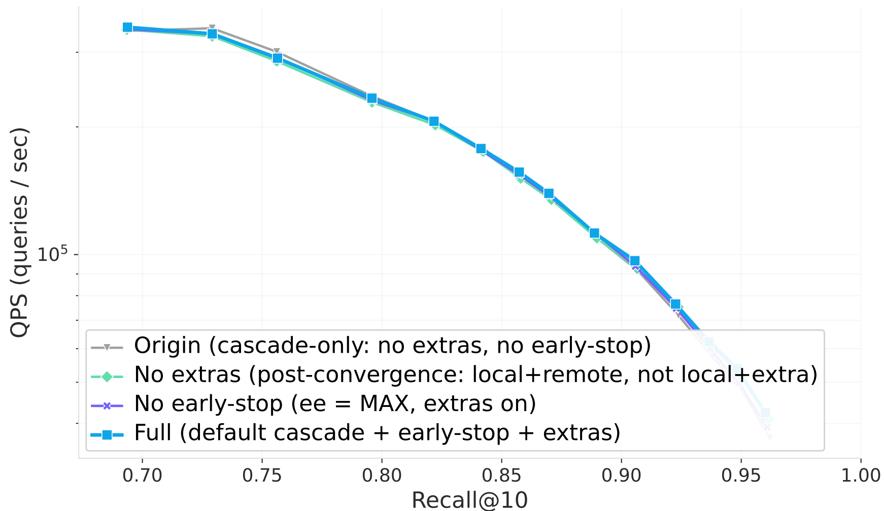
GloVe-100 (cosine) — Convergence-side ablation (8 threads, k=10) default cascade: None → MipsI8 → IpF32
