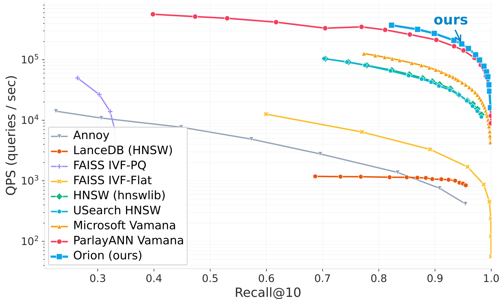
Deep10M — QPS vs Recall@10 (8 threads, k=10)
