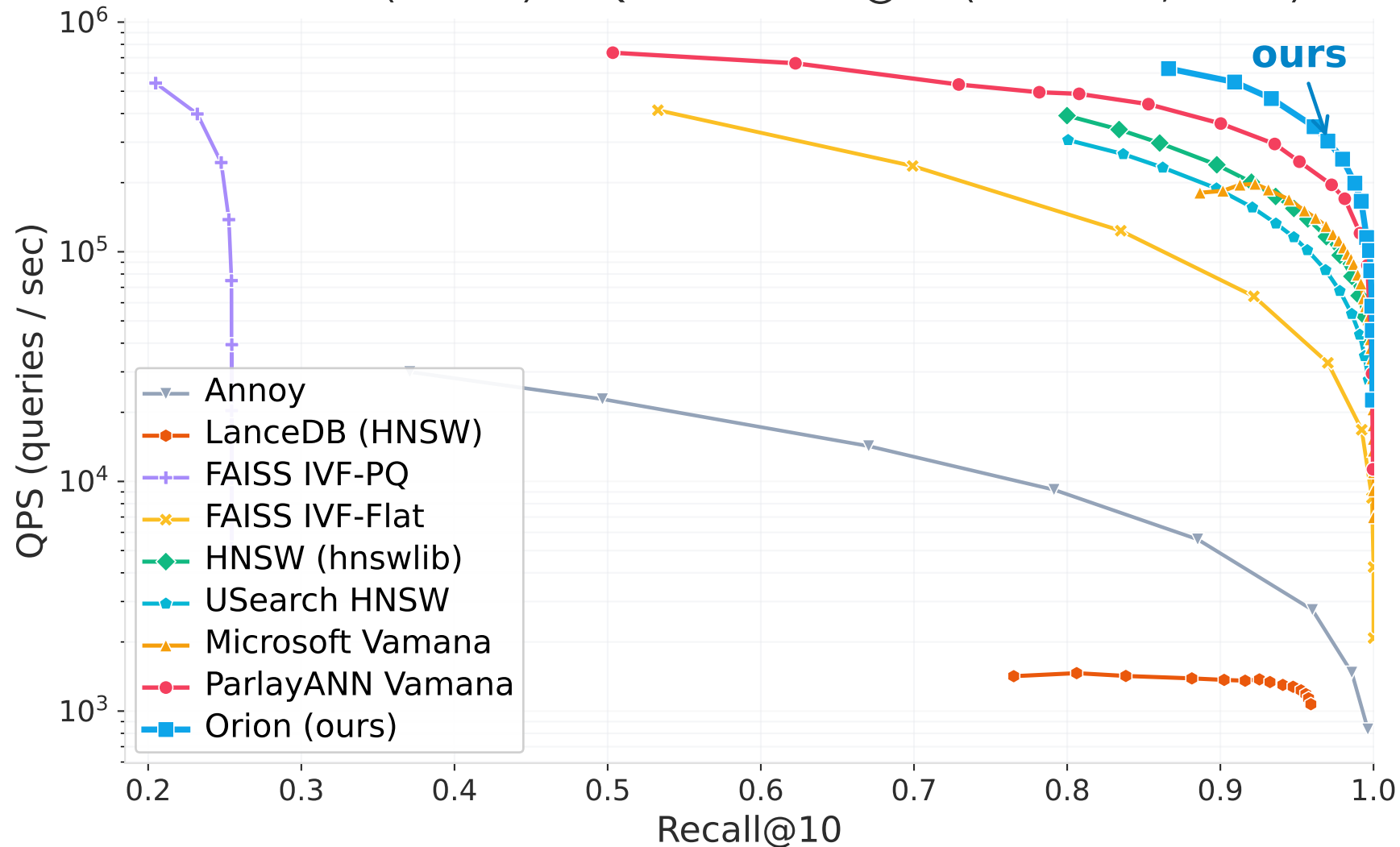
GloVe-25 (cosine) — QPS vs Recall@10 (8 threads, k=10)
