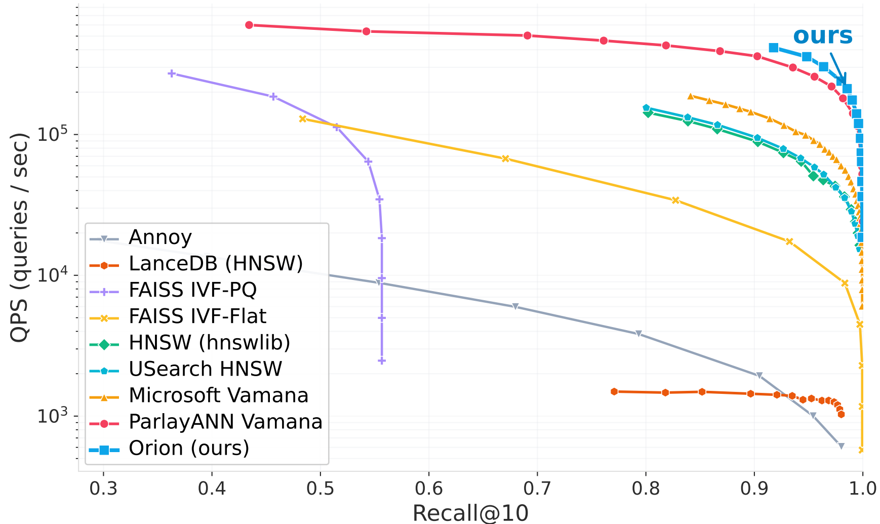
SIFT 1M — QPS vs Recall@10 (8 threads, k=10)
