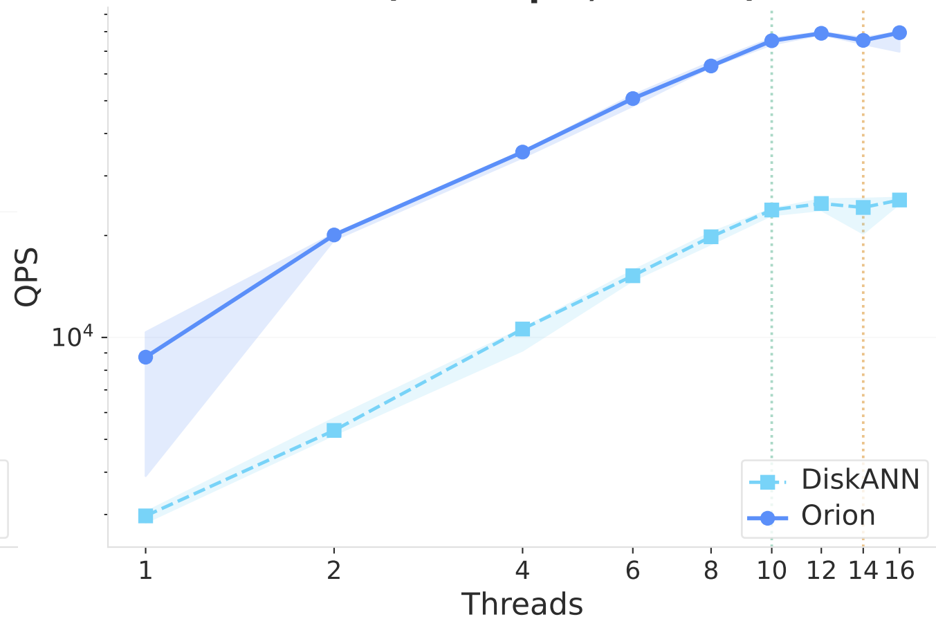
GIST (1000K pts, 5 trials)
