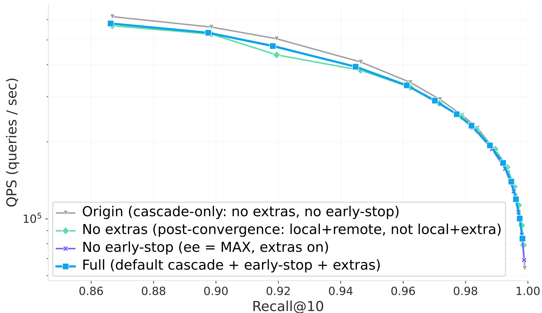
GloVe-25 (cosine) — Convergence-side ablation (8 threads, k=10) default cascade: None → MipsI8 → IpF32
