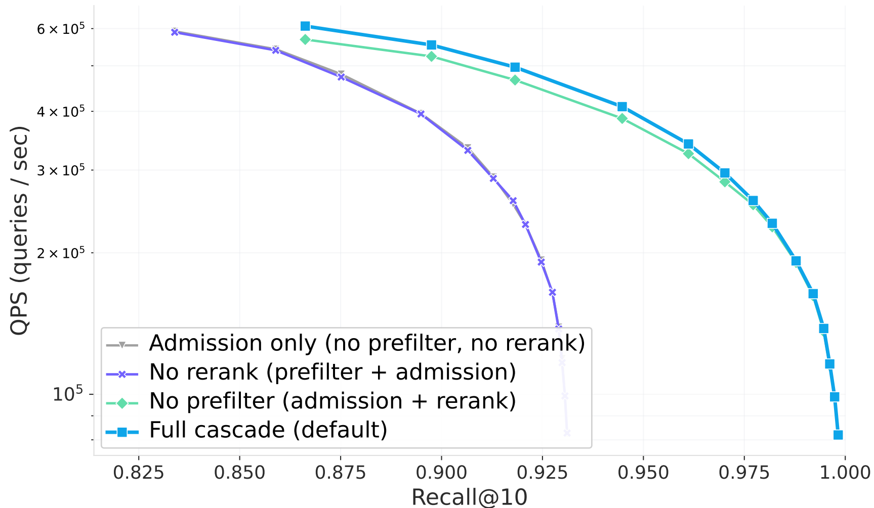
GloVe-25 (cosine) — Cascade-stage ablation (8 threads, k=10) default: None → Mips18 → IpF32
