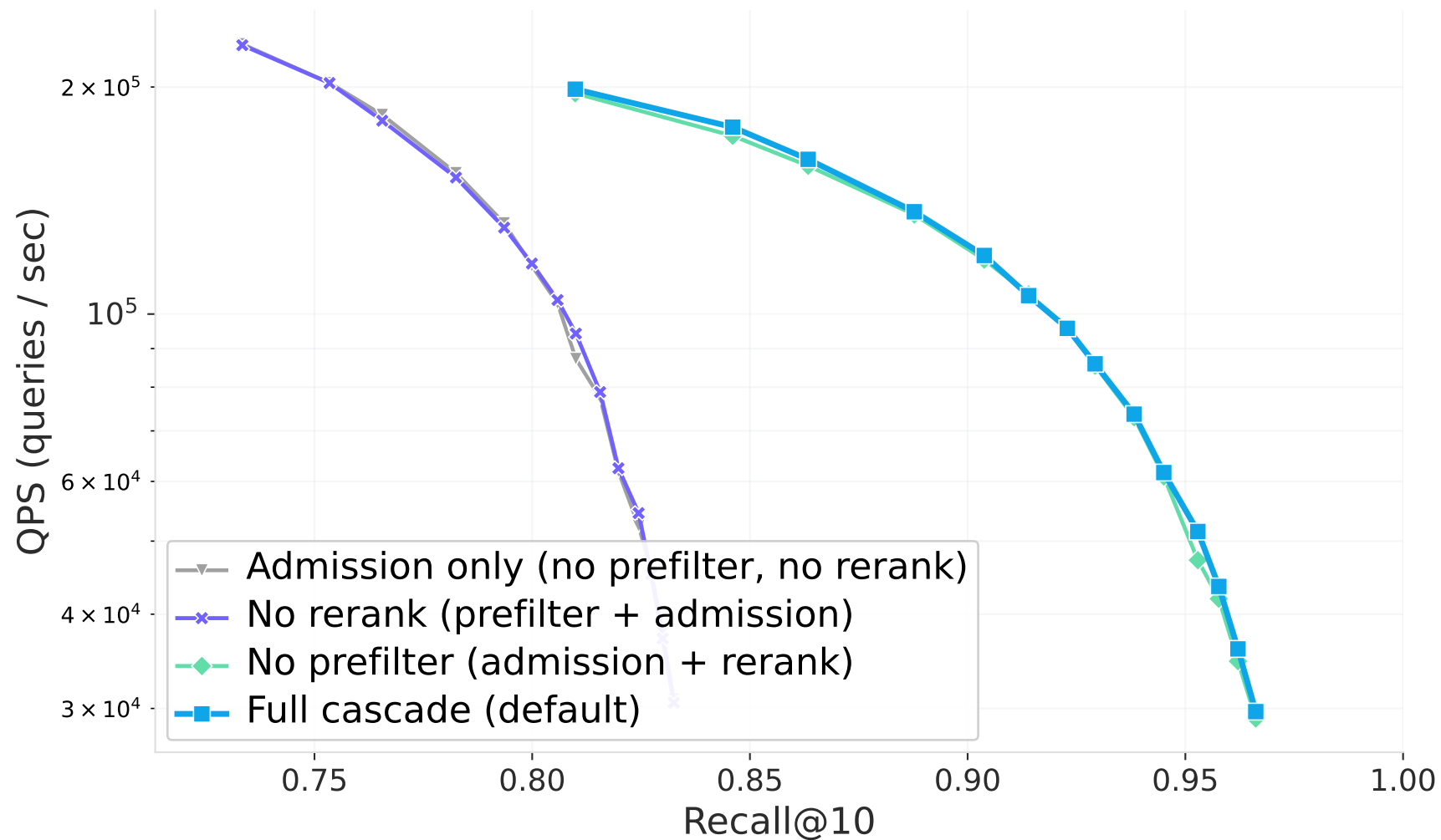
msmarco_bert_1M — Cascade-stage ablation (8 threads, k=10) default: None → MipsI8 → IpF32
