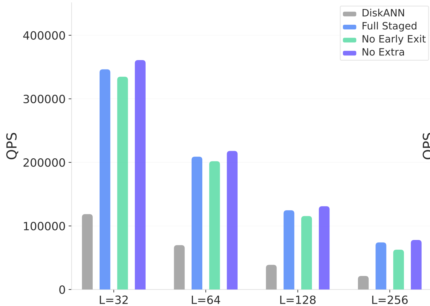
SIFT (128-dim) (1000K, 8T)
