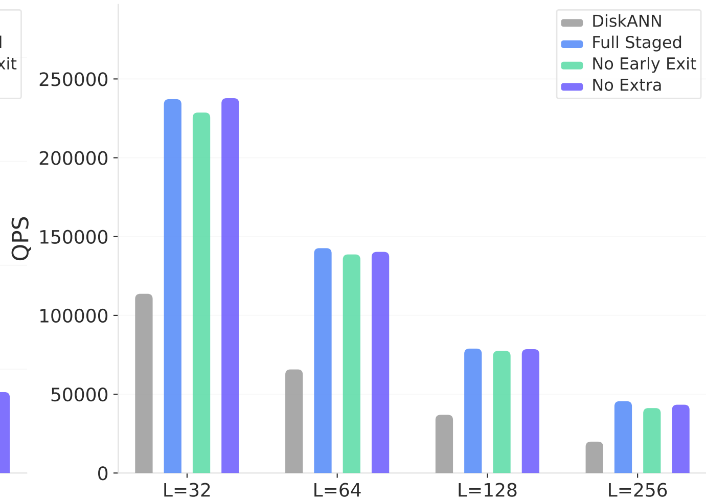
GloVe-100 (100-dim) (1183K, 8T)
