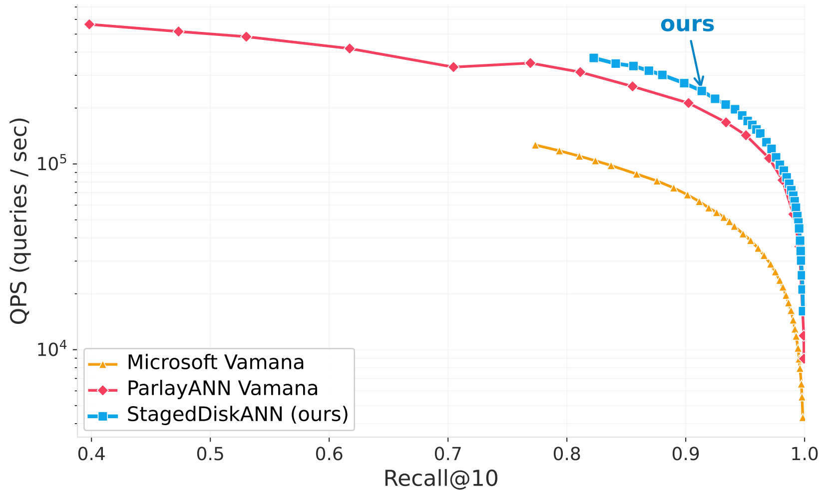
Deep10M — QPS vs Recall@10 (8 threads)
