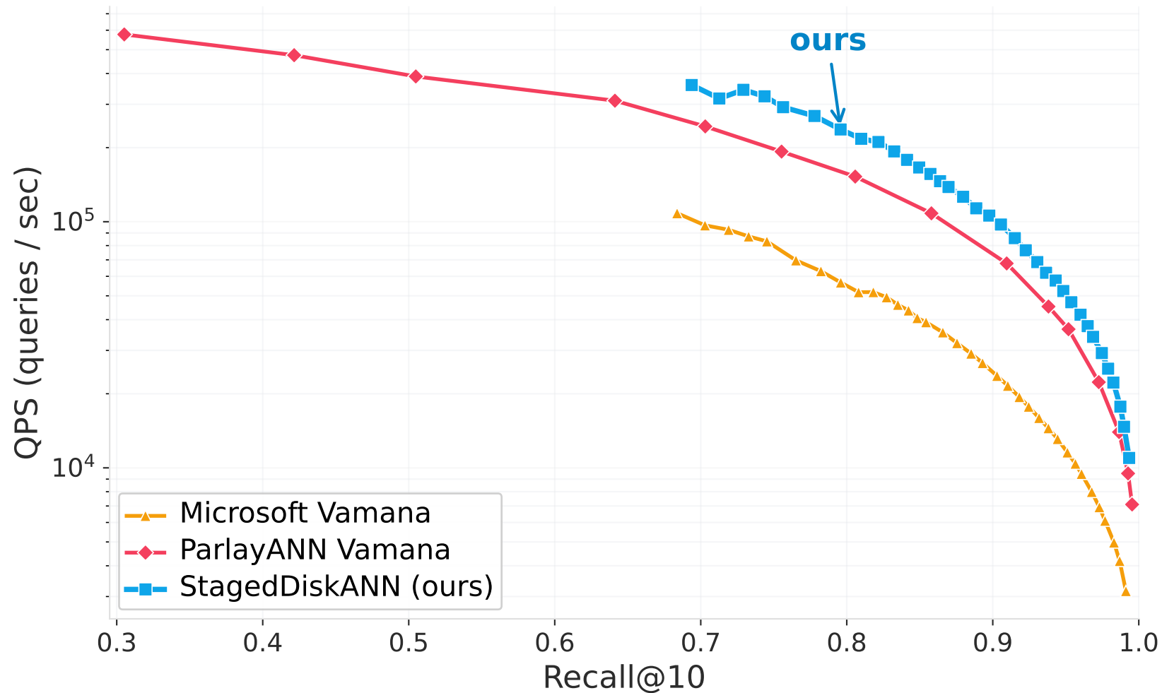
GloVe-100-angular — QPS vs Recall@10 (8 threads)
