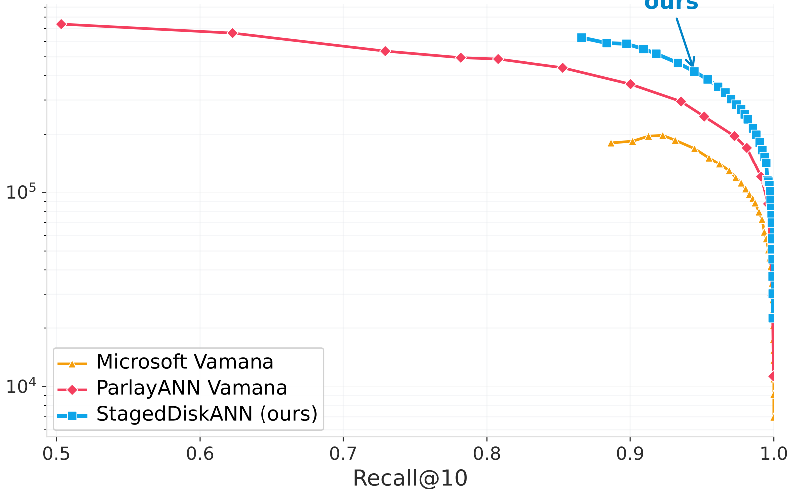
GloVe-25-angular — QPS vs Recall@10 (8 threads)
