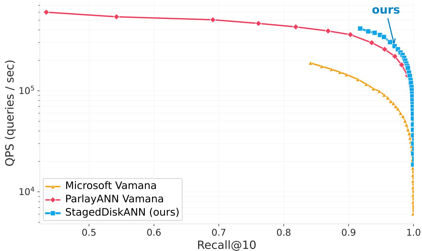
SIFT1M — QPS vs Recall@10 (8 threads)
