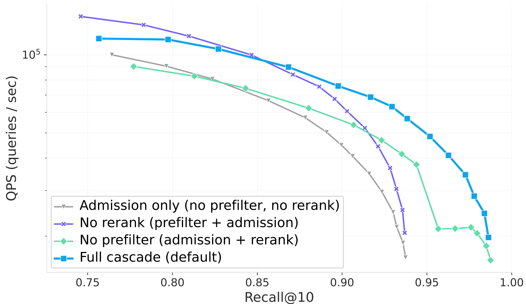
GIST 1M — Cascade-stage ablation (8 threads, k=10) default: JI → L2Kt → F32
