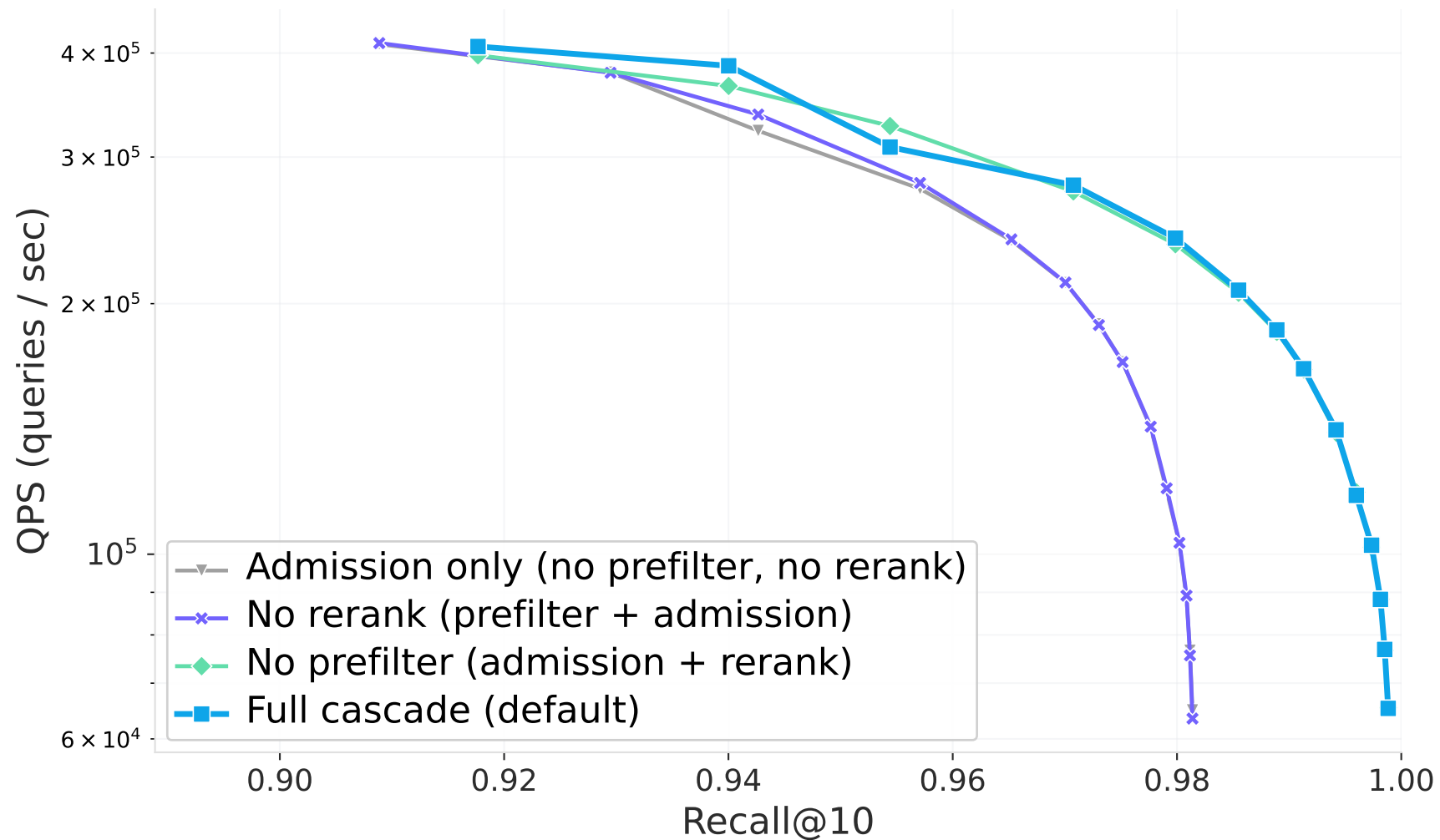
SIFT 1M — Cascade-stage ablation (8 threads, k=10) default: None → L2U8 → F32
