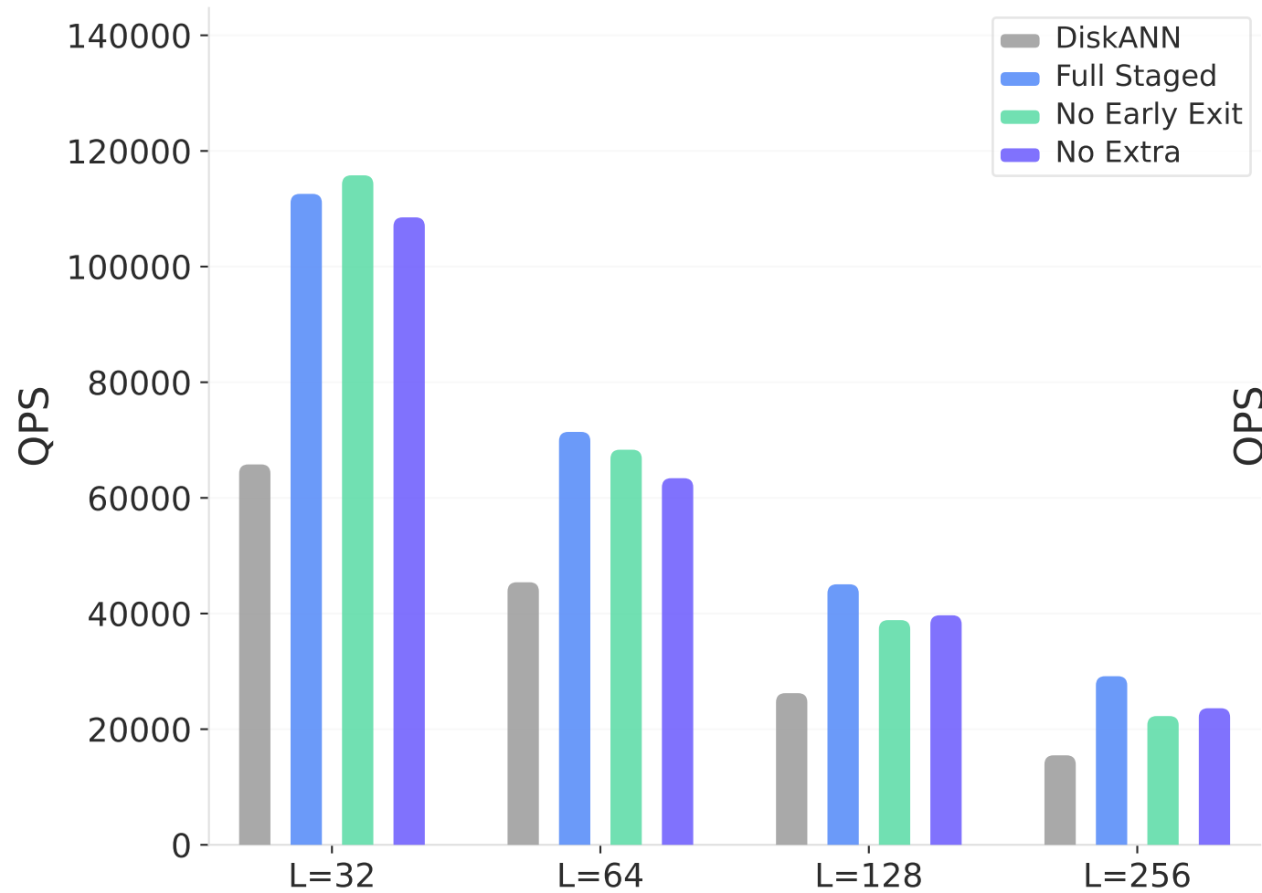
SIFT (128-dim) (100K, 8T)
