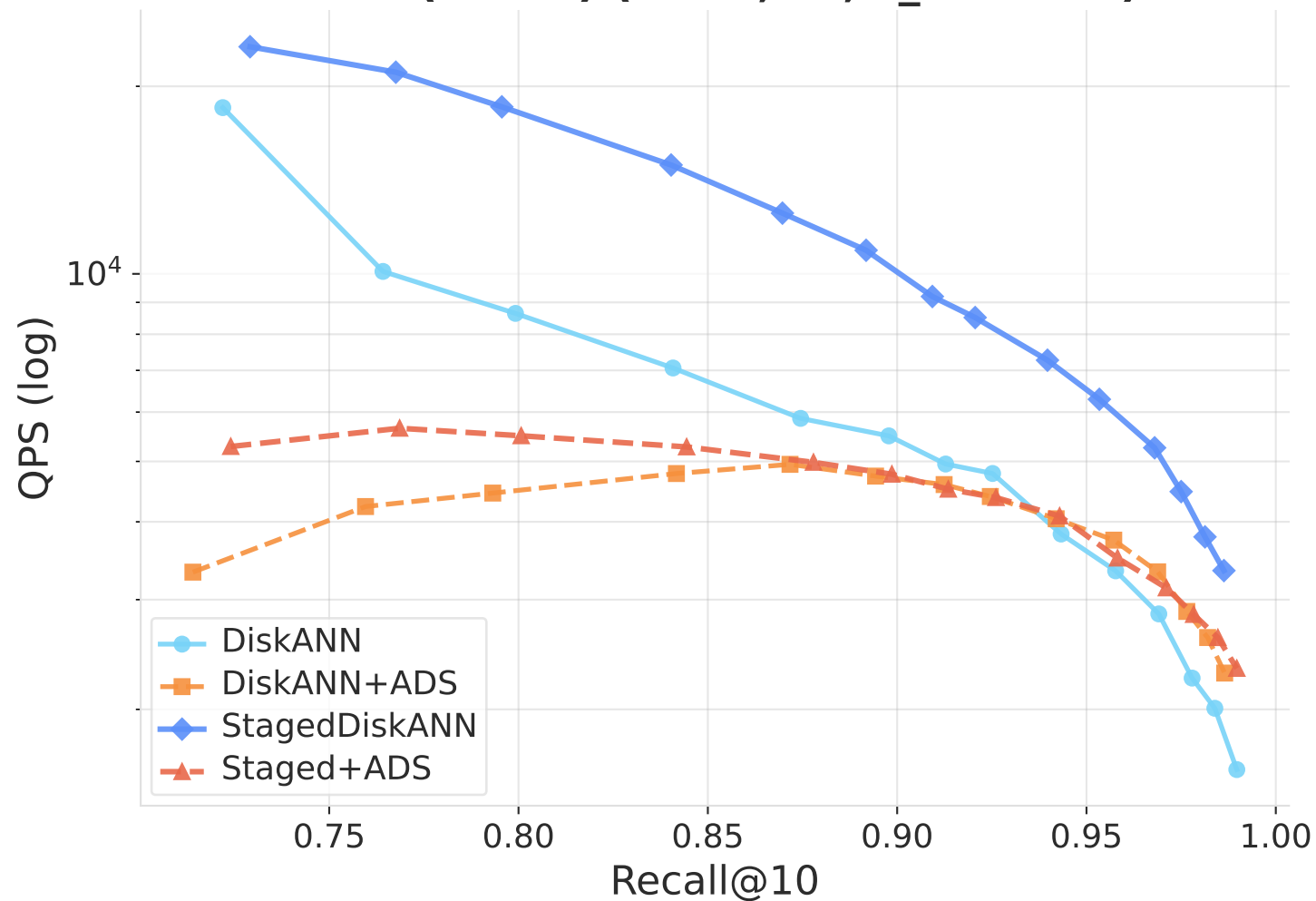
GIST (960-d) (100K, 8T, \epsilon_{\text{ads}}=2.1 )
