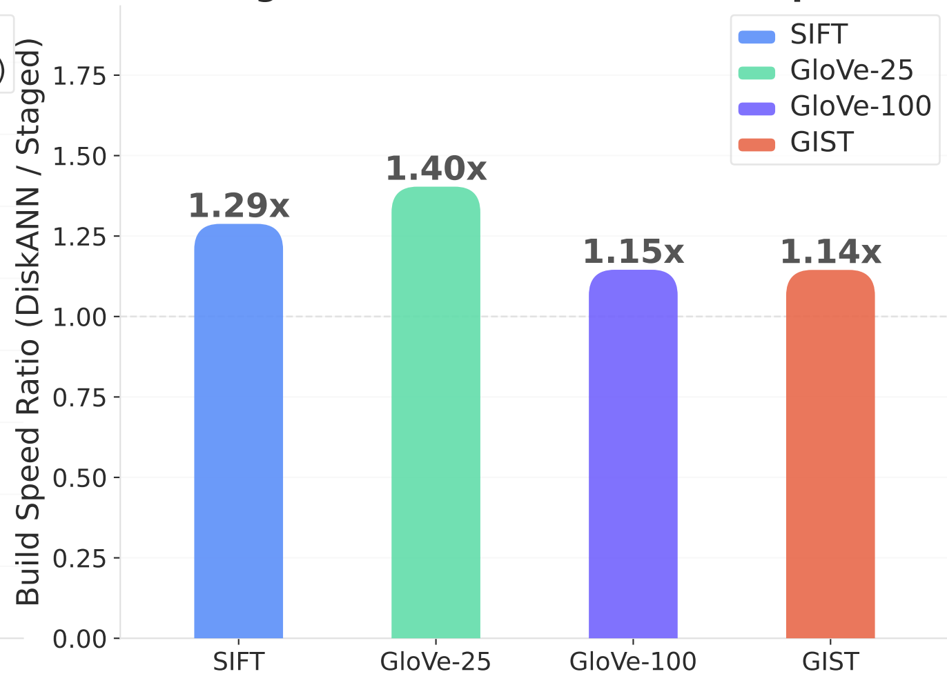
Staged Build is Faster (Lower Alpha)
