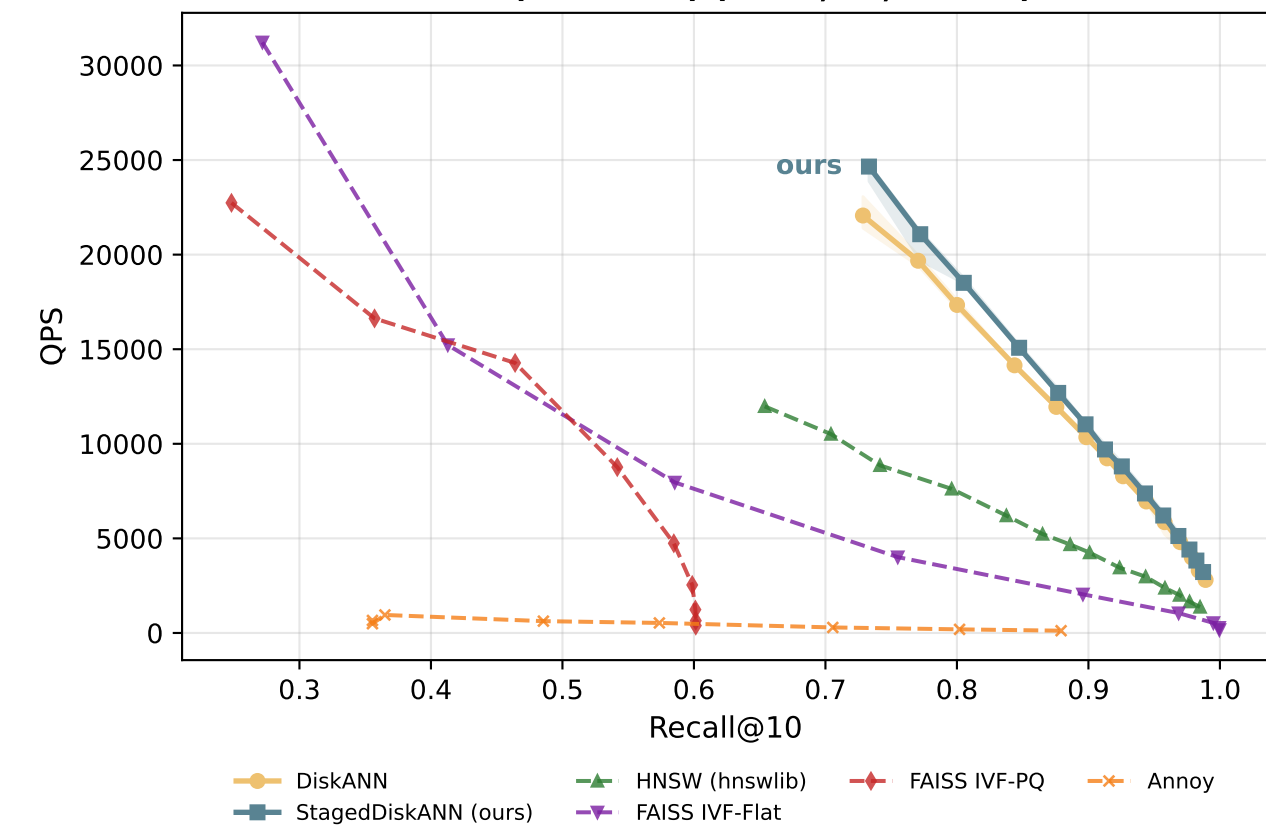
GIST (dim=960) (100K, 8T, 3 runs)
