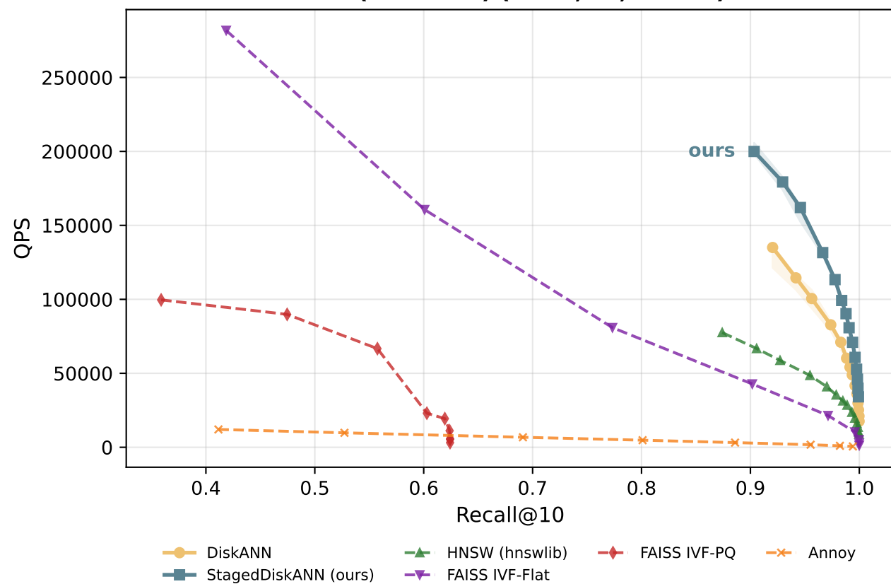
SIFT (dim=128) (100K, 8T, 3 runs)
