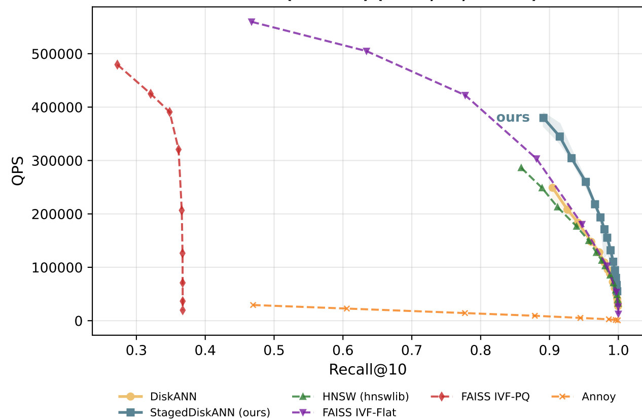
GloVe-25 (dim=32) (100K, 8T, 3 runs)
