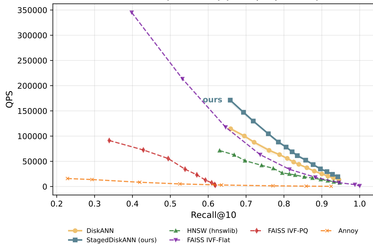
GloVe-100 (dim=100) (100K, 8T, 3 runs)
