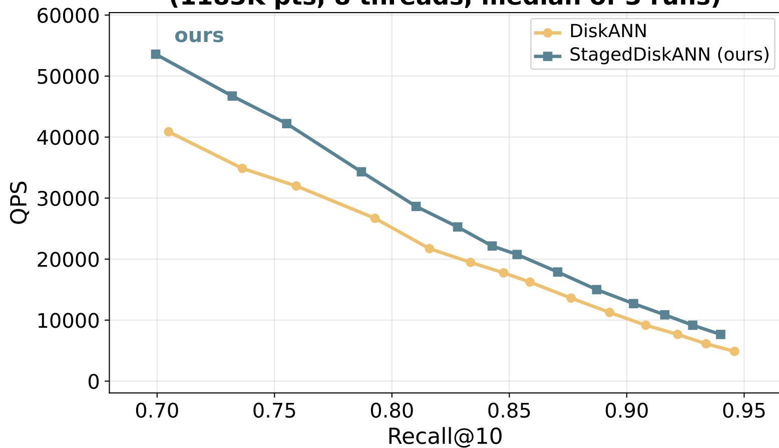
GLoVe-100 (dim=100) (1183K pts, 8 threads, median of 3 runs)
