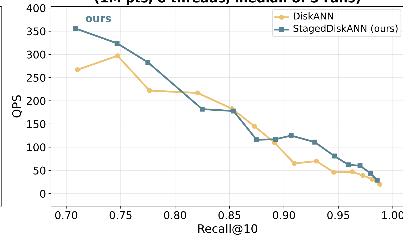
GIST (dim=960) (1M pts, 8 threads, median of 3 runs)
