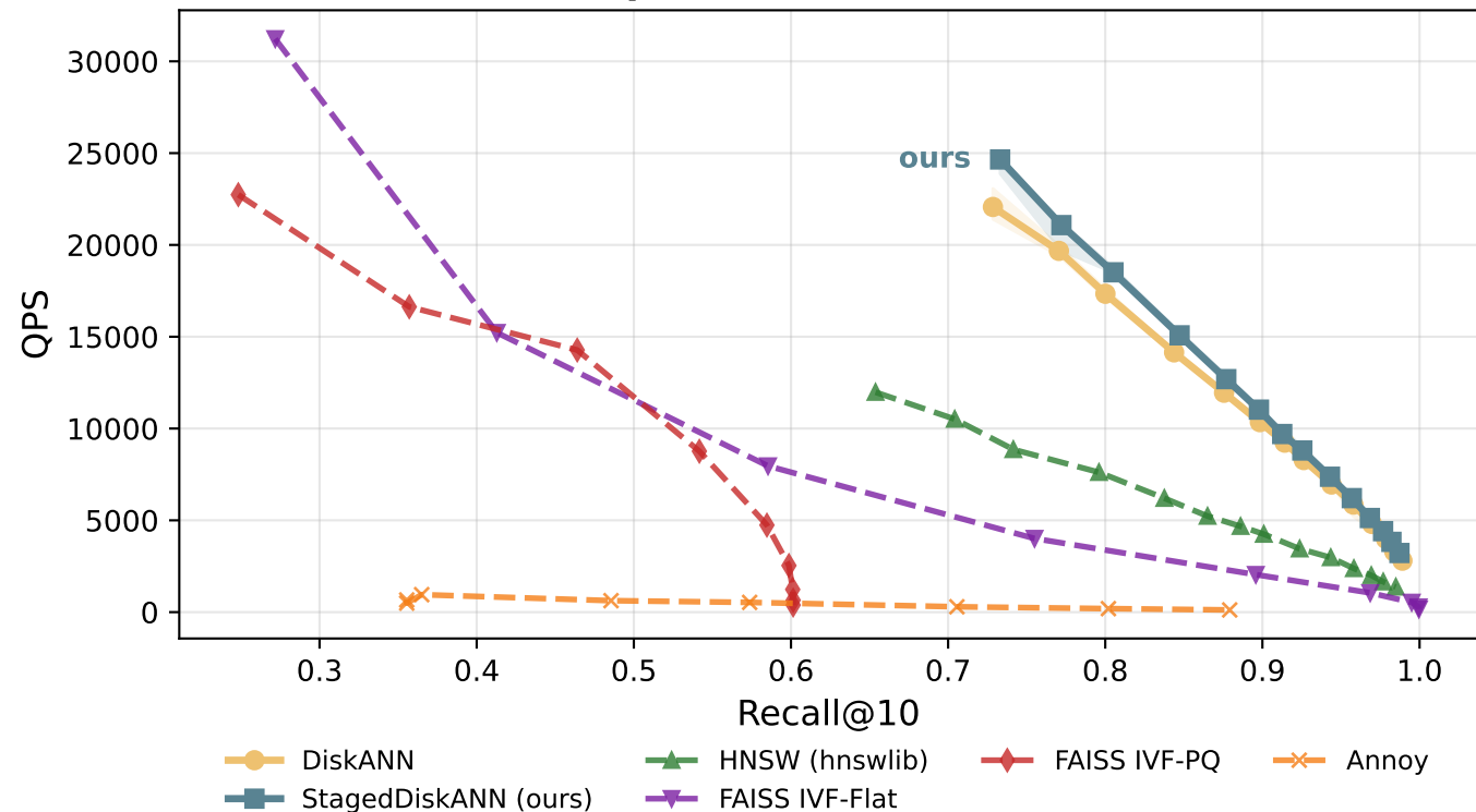
QPS vs Recall@10 -- GIST (dim=960) (100K points, 8 threads, 3 runs)
