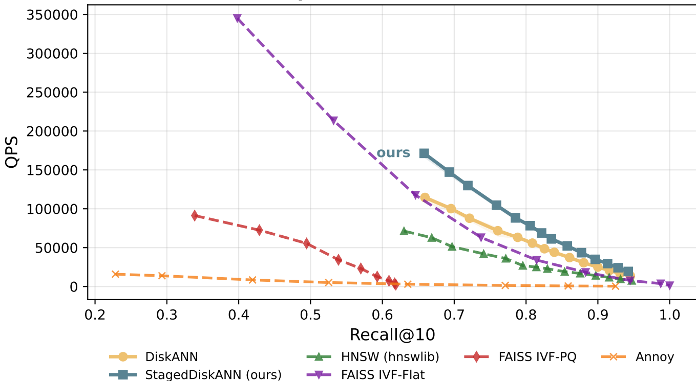
QPS vs Recall@10 -- GloVe-100 (dim=100) (100K points, 8 threads, 3 runs)
