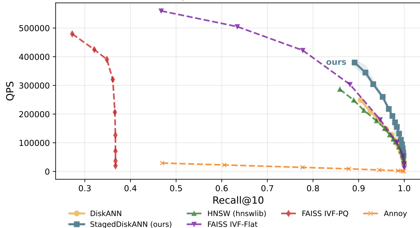
QPS vs Recall@10 -- GloVe-25 (dim=32) (100K points, 8 threads, 3 runs)
