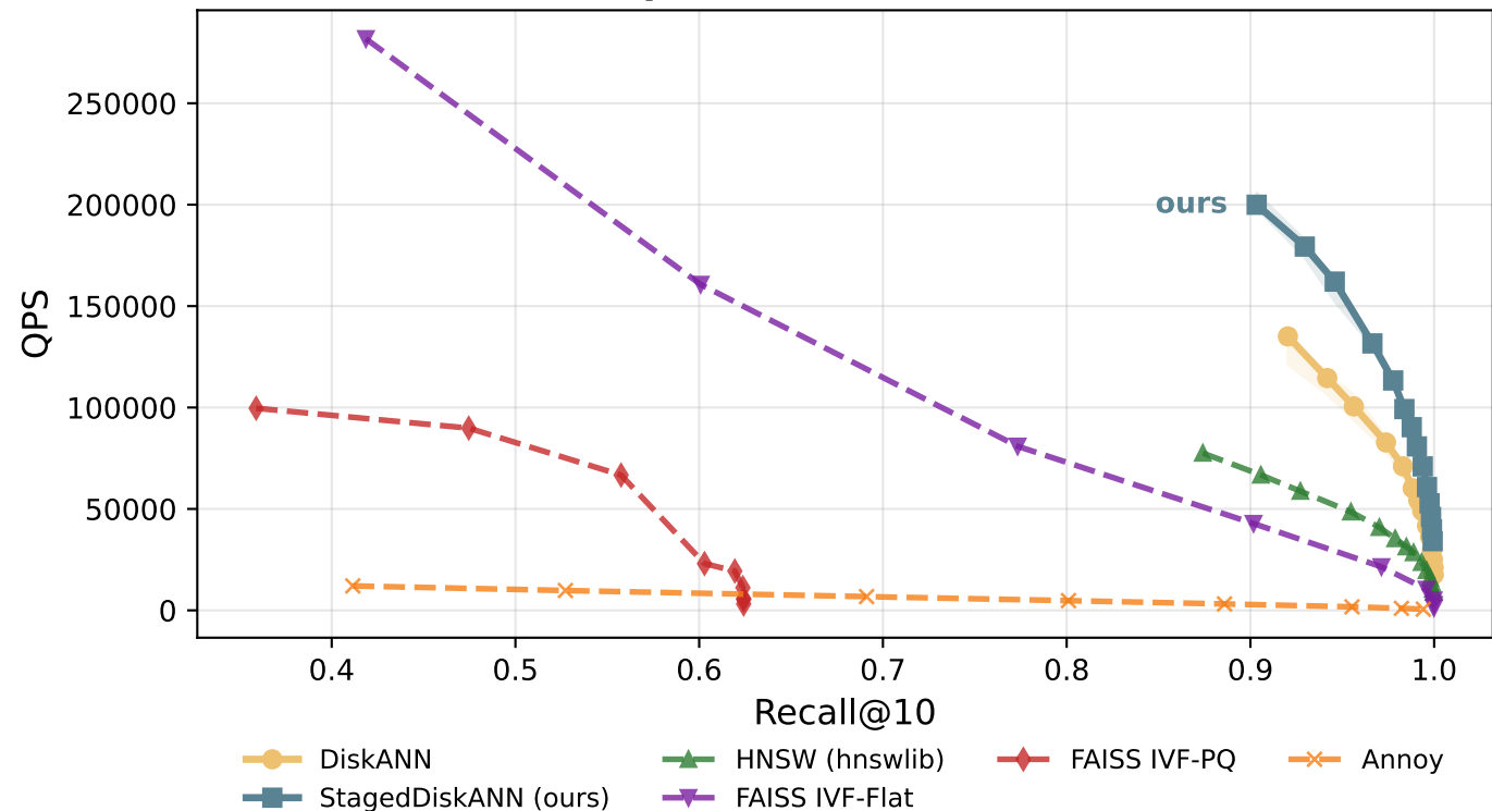
QPS vs Recall@10 -- SIFT (dim=128) (100K points, 8 threads, 3 runs)
