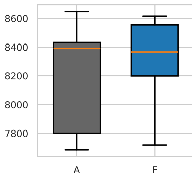
Gen-Insert
