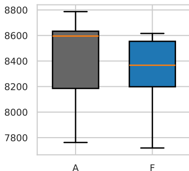
Reorder
