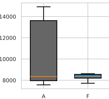
Splice
