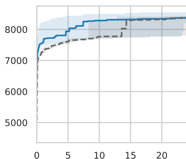
Gen-Insert
