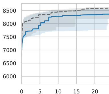
Reorder
