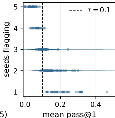
(c) Boundary mass
