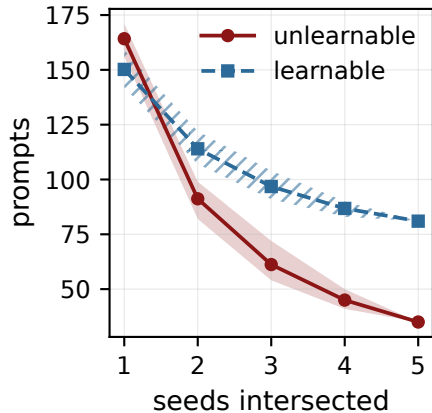
(a) Set size vs seed count
