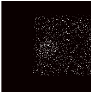
merged_soft.fits
