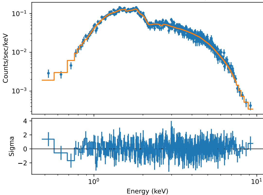
Simulated spectrum and fit without pile-up
