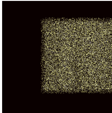
acis7s_bkg_reproj.fits
