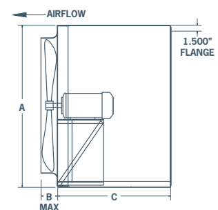
DIRECT DRIVE
