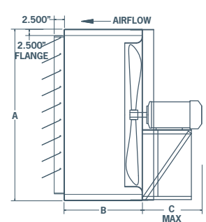
DIRECT DRIVE
