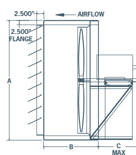
BELT DRIVE
